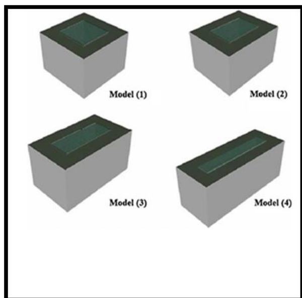
Figure I. 7 : Variations de la géométrie des types d'atriums. Source : Abdelsalam, A. The influence of the atrium geometry on the building energy performance, Energy and Buildings, Volume 57, February 2013.
