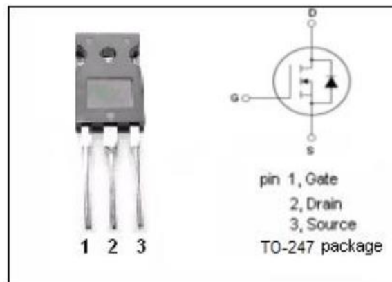
Figure III-2: IRFP260M Transistor
