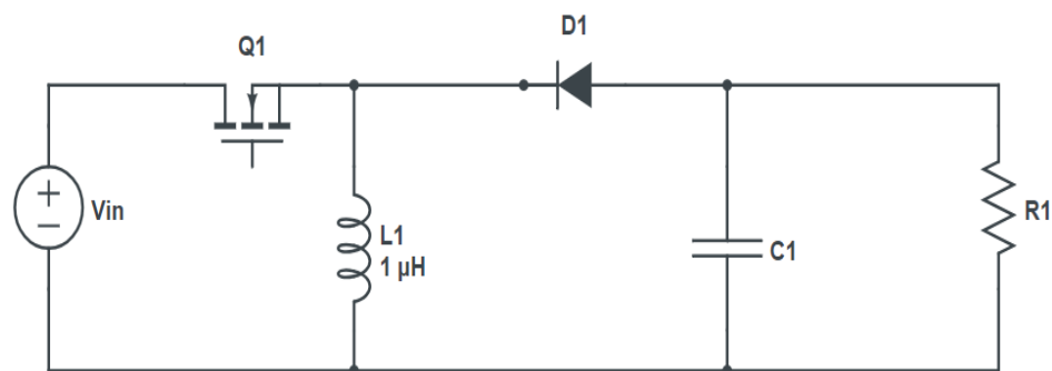
Figure I-4: Buck-Boost converter
