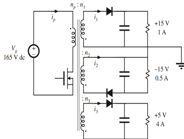
Figure II-1: Flyback converter multiple outputs
