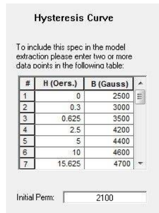
Figure III-12:the hysteresis filled table
