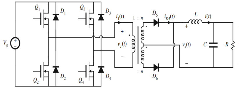
Figure I-7: Full-bridge circuit
