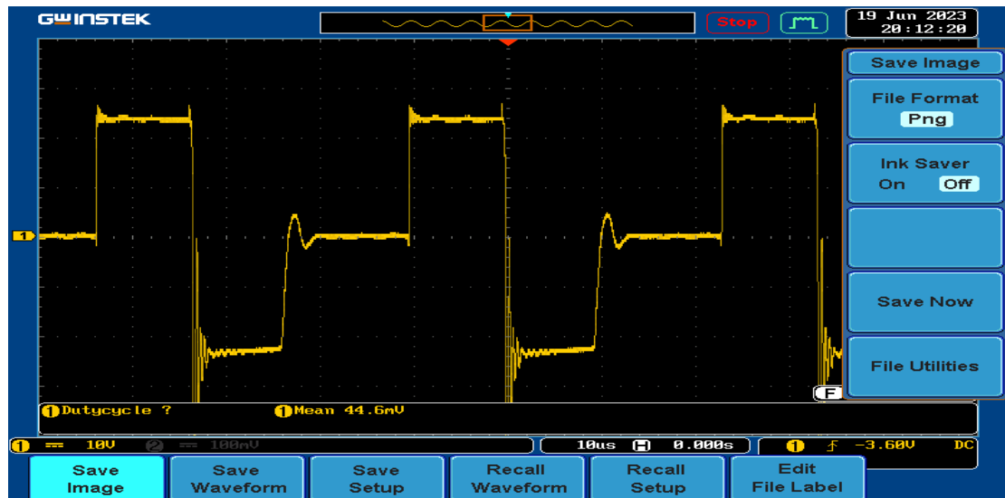
Figure III-22: primary winding voltage
