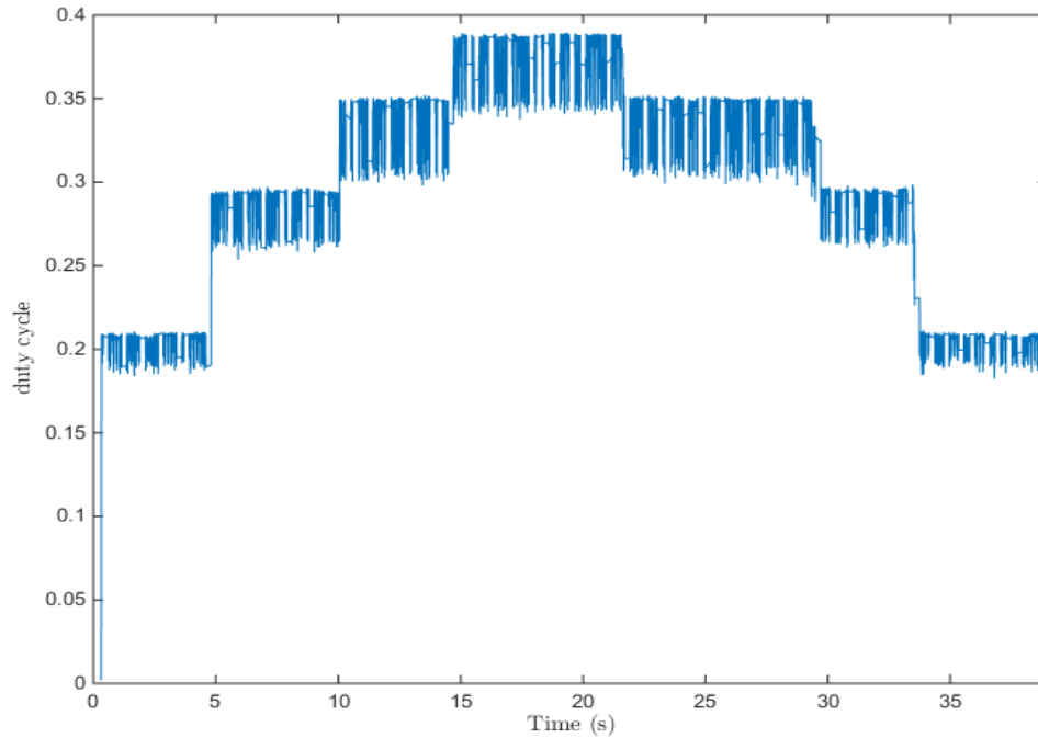
Figure III-35:Duty cycle test 2
