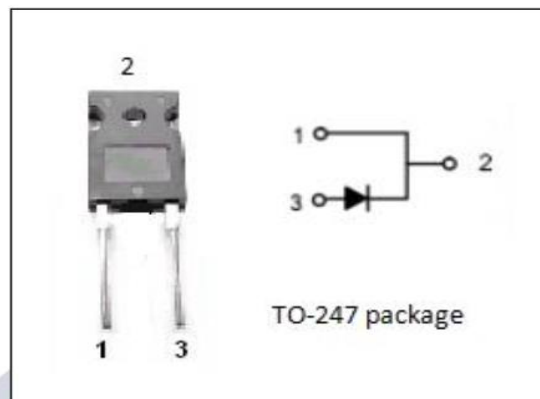
Figure III-3: RHRG75120 Diode
