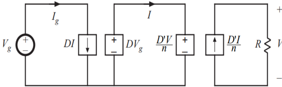
Figure II-5: Flyback converter equivalent circuit model
