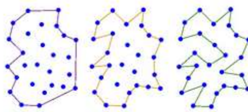
Figure 6. Diverses enveloppes concaves possibles
