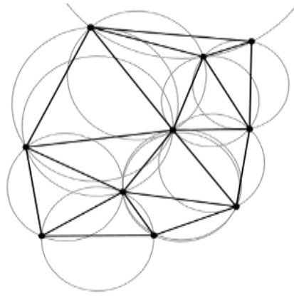
Figure 7. Triangulation de Delaunay [41]
