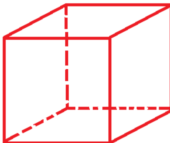
Figure 4. Cube
