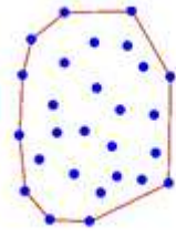
Figure 5. Enveloppe convexe
