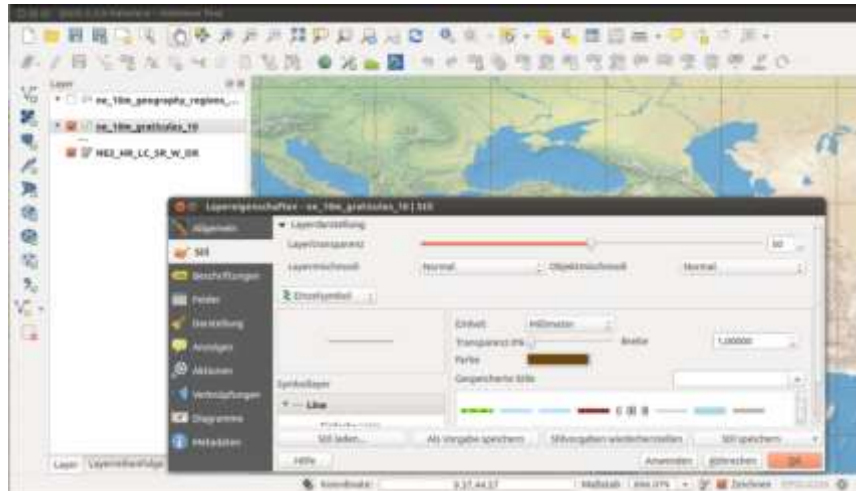
Figure 2-Interface QGIS [8]
