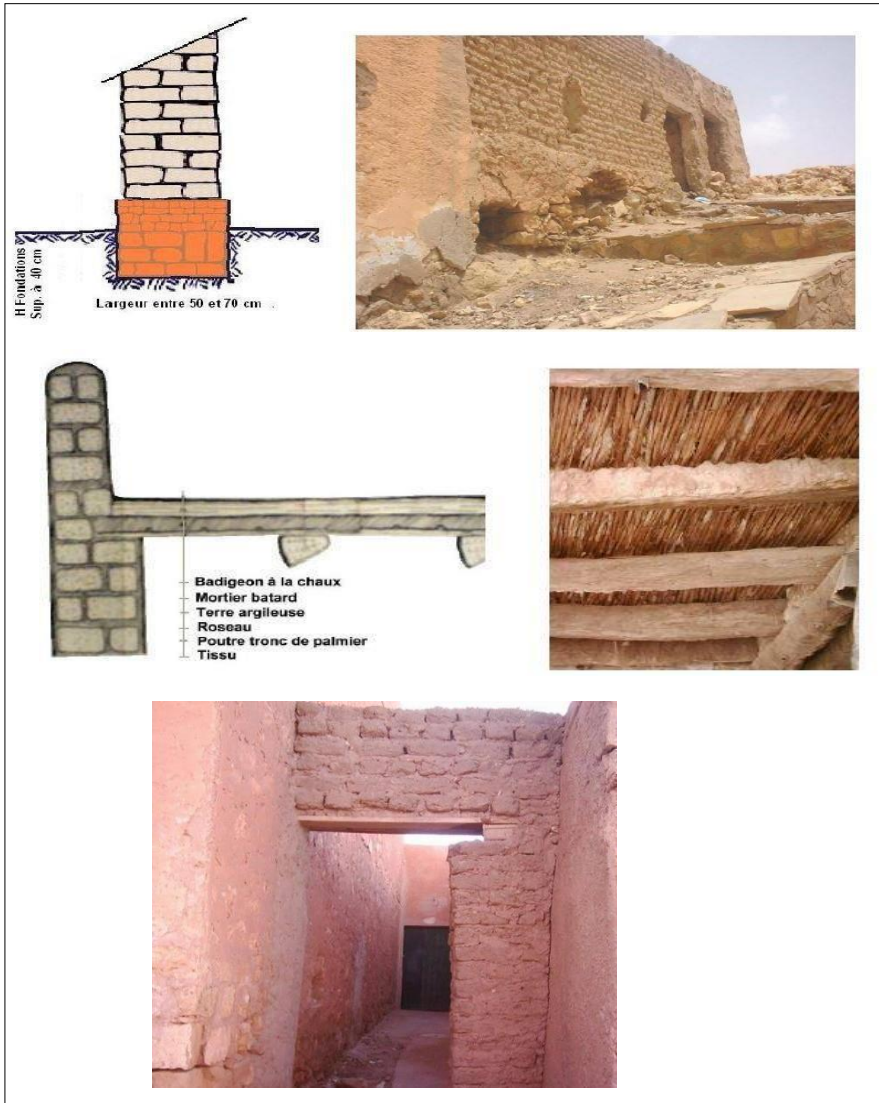
FIG 27 TECHNIQUES DE CONSTRUCTION Source: KERROUM Nadir, Op. Cit.
